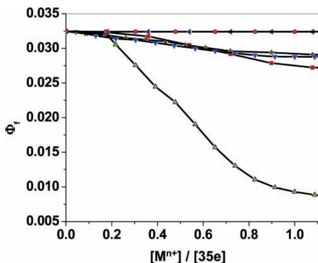
FIGURE 12. Plot of \Phi_f versus the ratio between metal ion and 35e , which illustrates the selectivity for \text{Ca}^{2+} ( \blacktriangle ) over \text{Na}^+ (tilted \blacktriangle ), \text{K}^+ ( \bullet ), \text{Mg}^{2+} ( \blacksquare ), \text{Sr}^{2+} ( \blackstar ), and \text{Ba}^{2+} ( \blacktriangledown ) (adapted from ref 41).
